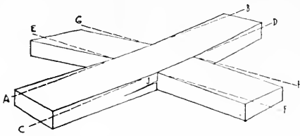
FIG. 246. SHOWING RESULTS OF FORCING FIT IN LAP-JOINT.
